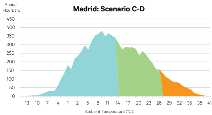
Figure 7. Madrid profile: With optimized chilled water system control, improved compressor technology and low-GWP refrigerant
