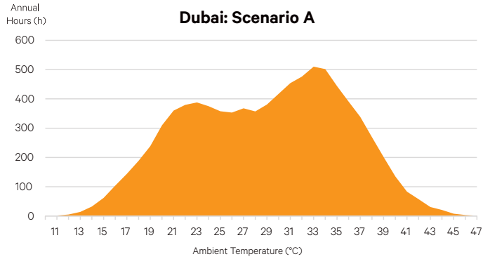
Figure 9. Dubai profile: Traditional Chilled Water System
