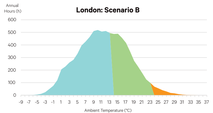
Figure 2. London profile: With increased air and water temperatures
