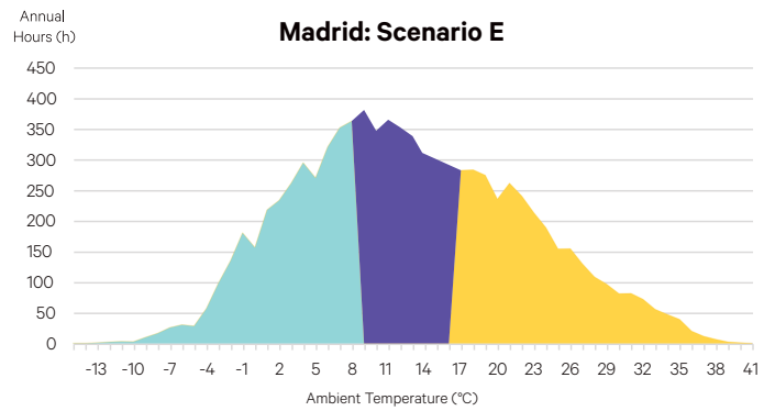
Figure 8. Madrid profile: Including the adiabatic system
