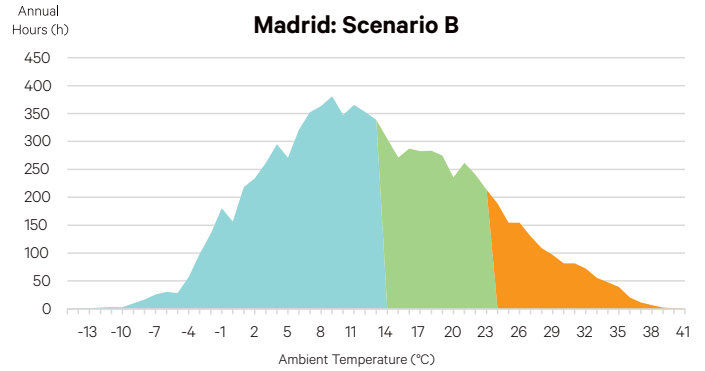
Figure 6. Madrid profile: With increased air and water temperatures
