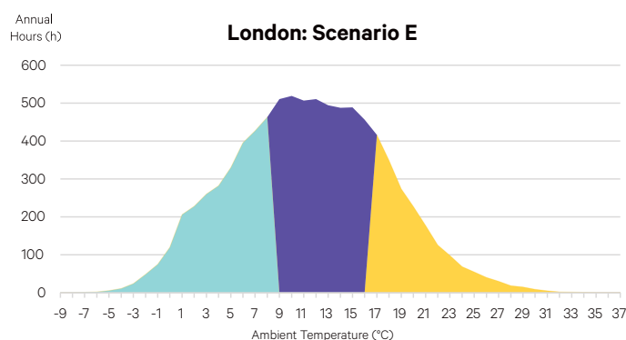
Figure 4. London profile: Including the adiabatic system
