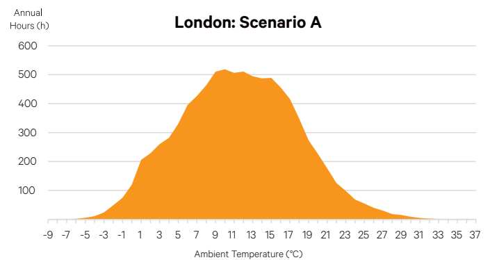
Figure 1. London profile: Traditional Chilled Water System
