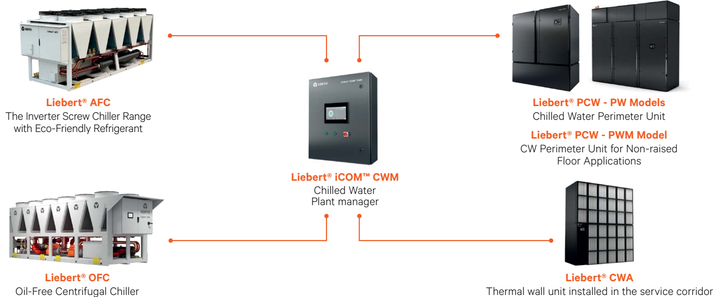
Figure 1. Vertiv's Enlarged Portfolio for a State-of-the-Art Chilled Water System
