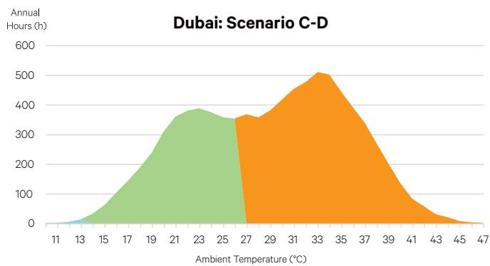
Figure 11. Dubai profile: With optimized chilled water system control, improved compressor technology and low-GWP refrigerant
