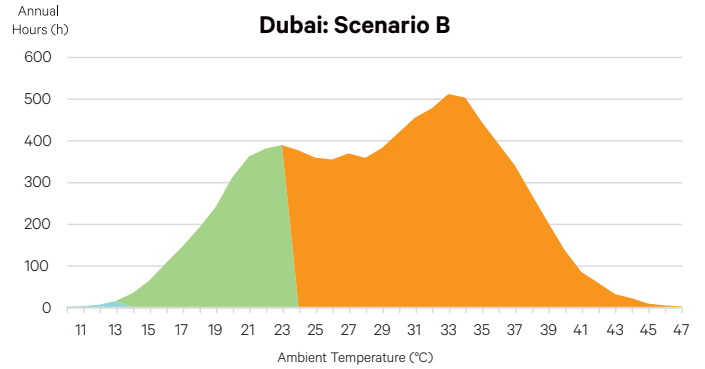
Figure 10. Dubai profile: With increased air and water temperatures
