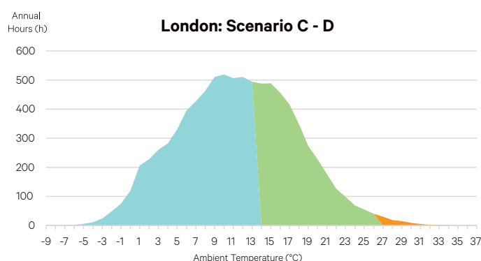
Figure 3. London profile: With optimized chilled water system control, improved compressor technology and low-GWP refrigerant
