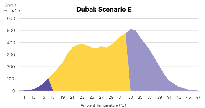
Figure 12. Dubai profile: Including the adiabatic system
